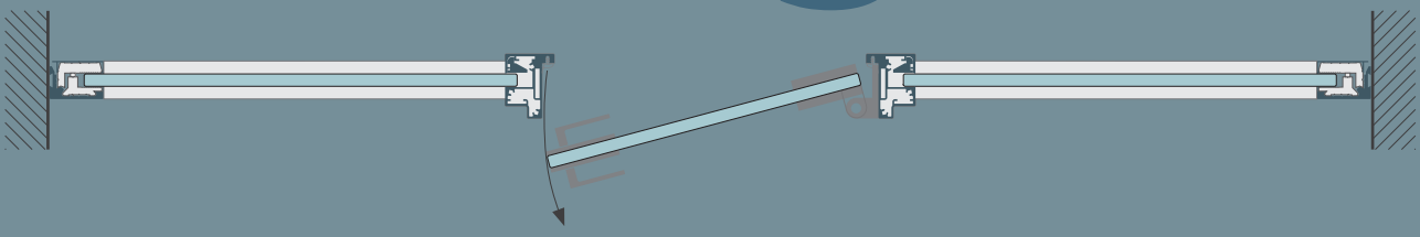
SOLID DOOR LEAF IN THE DOOR JAMB /SWING/
