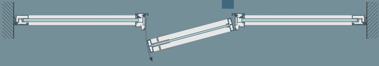
DOOR LEAF IN THE ALU 1 PROFILE /SWING/
