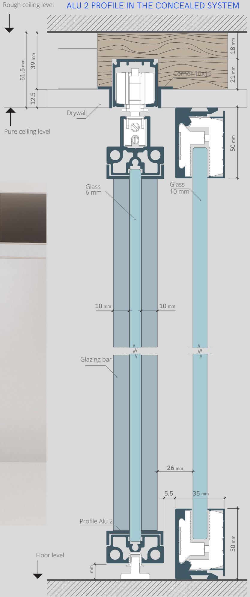
Hafele SLIDO CLASSIC - I system
