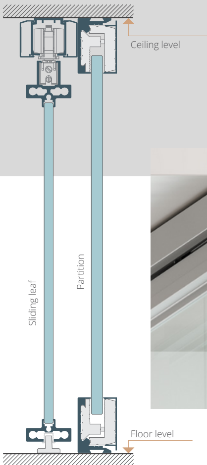
SECTION 1-1
