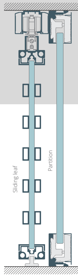
SECTION 2-2
