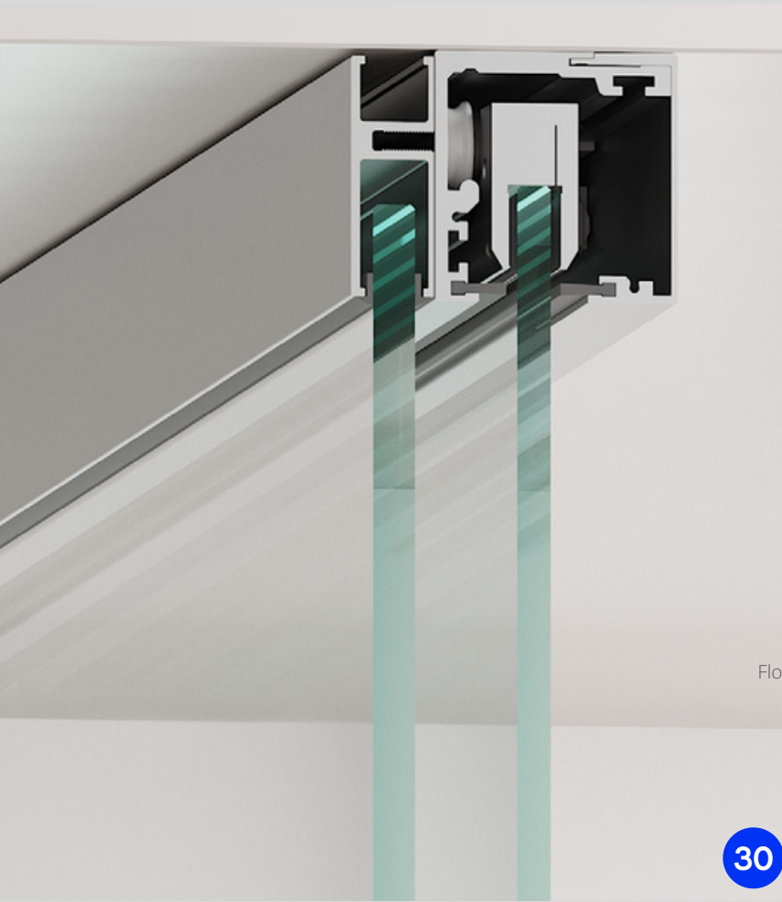
Hafele SLIDO CLASSIC - F system
