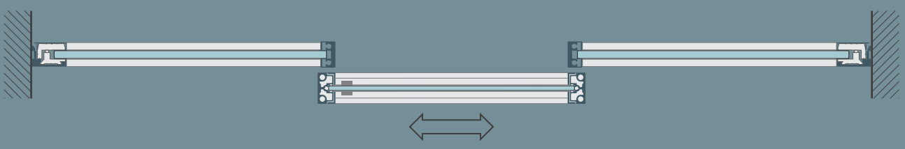
ALU 2 DOOR LEAF WITH THE GLAZING BARS /SLIDING/ 2
